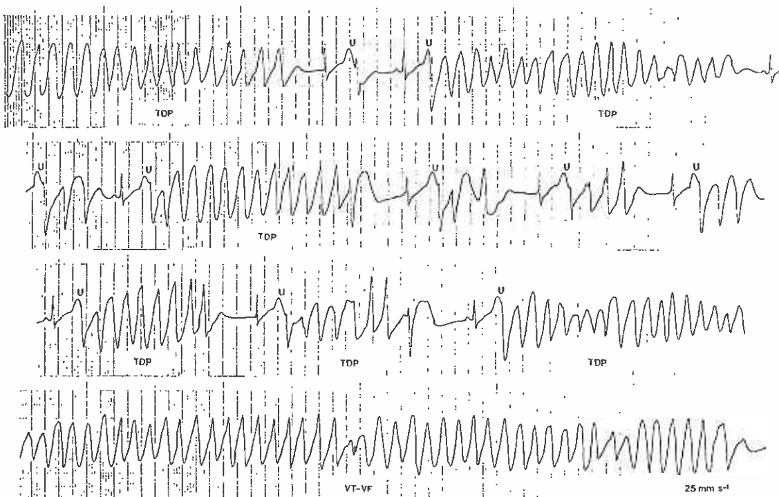
Fig 3 - Pre-terminal ECG: Continuous recording showing repetitive runs of torsade de pointes (TDP) - variable paroxysms of which terminated spontaneously. The late cycle phases of the very prominent post-pause U waves appeared to be the foci of origin of the torsade de pointes. The rate for the TDP varied from 240 to 280 beats per minute. The QTU (uncorrected) interval averaged 0.45 second. (Note that there seemed to be a correlation between the length of the post-pause duration and the accentuation of the U waves.) The final prolonged salvo of TDP deteriorated into a ventricular tachycardia-fibrillation (VT-VF).
